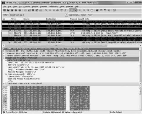
图：Wireshark ( http://www.wireshark.org/ )
